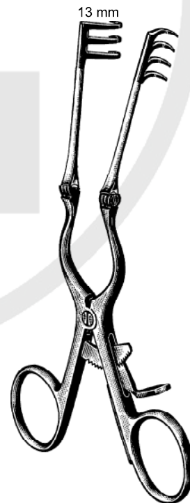
Weitlaner-Beckmann 389-11 16.5 cm / 6 1/2" Sharp 389-12 16.5 cm / 6 1/2" Blunt 389-13 20 cm / 8" Sharp 389-14 20 cm / 8" Blunt 3 X 4 Prongs
