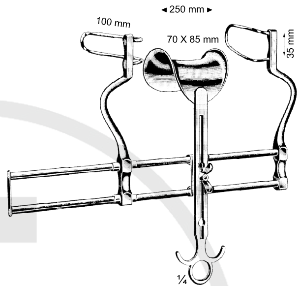
Balfour 406-03 Opening 250 mm Wire blades 35 X 100 mm 406-04 Opening 280 mm 40 X 105 mm 406-05 Opening 300 mm 40 X 110 mm
